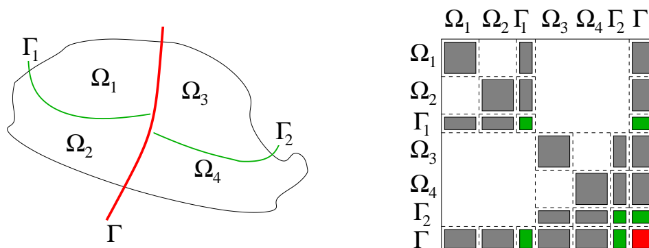
FIGURE 1. Nested dissection and resulting matrix sparsity structure
