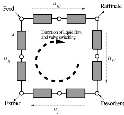
FIGURE 1. Standard SMB process with two columns in each zone
