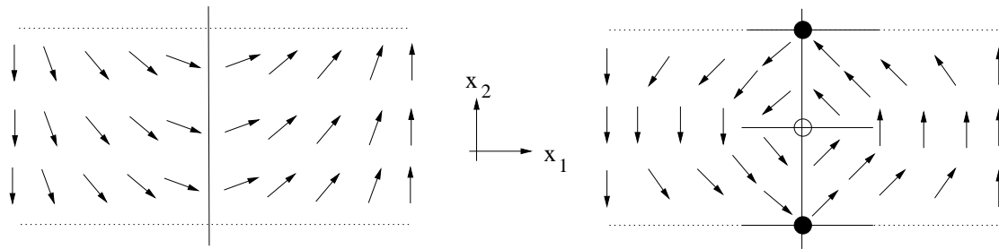
FIGURE 2. Néel wall and cross-tie wall
