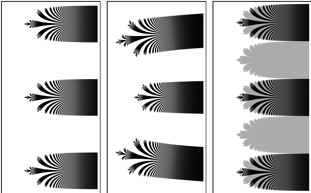
FIGURE 1. Three Julia sets of different entire functions: the first is z \mapsto 2(\exp(z) - 1) , the second one is z \mapsto (z + 1)\exp(z) - 1 ; our results imply that these are quasiconformally conjugate on their Julia sets. The third picture shows a subset of the Julia set of a function of the form z \mapsto \lambda \sinh(z) on which this function is quasiconformally conjugate to the previous two.
