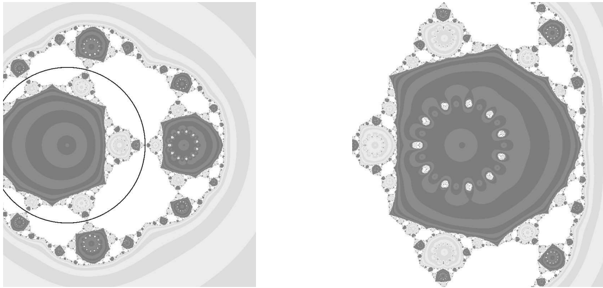
FIGURE 1. The Fatou sets of the mappings f_{c,\rho,\nu,\eta,\alpha} contain components of connectivity \nu + 1 : On the left hand side, a Fatou set containing 12-fold connected components ( c = 1.5 , \rho = 0.175 , \nu = 11 , \eta = 1 , \alpha = 0 ) is presented. On the right hand side a close-up view on the area [0.9, 2.1] + i[-1.05, 1.05] containing the multiply connected preimage of the immediate basin of attraction of 0 is given. The black circle on the left hand side represents the unit circle.
