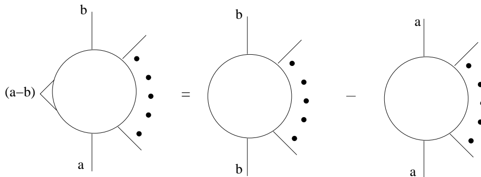
FIGURE 1. The Ward identity
