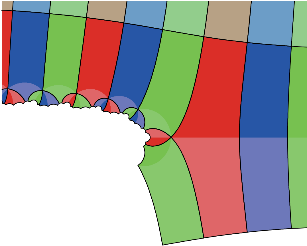
FIGURE 2. Truncated Checkerboard Pattern
