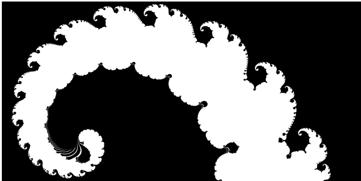
FIGURE 1. The Julia set of a Poincaré function \psi . Here \psi was normalized in a way that ensures that the Fatou set, shown in white, is a single immediate basin of attraction. The polynomial p is the center of the 1/15-limb of the Mandelbrot set.
