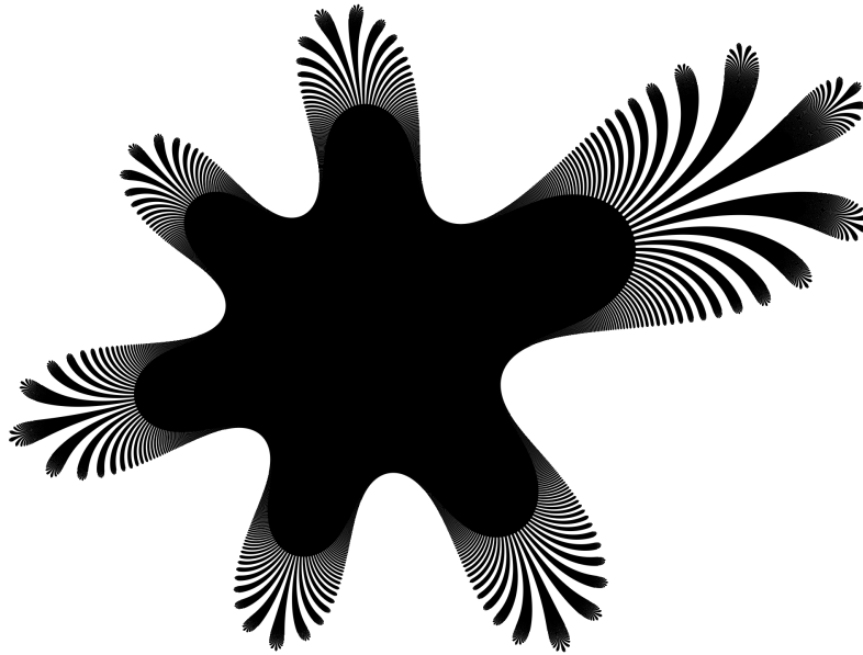
FIGURE 2. A nonlinearizable arithmetical hedgehog (picture courtesy of Arnaud Chéritat)
