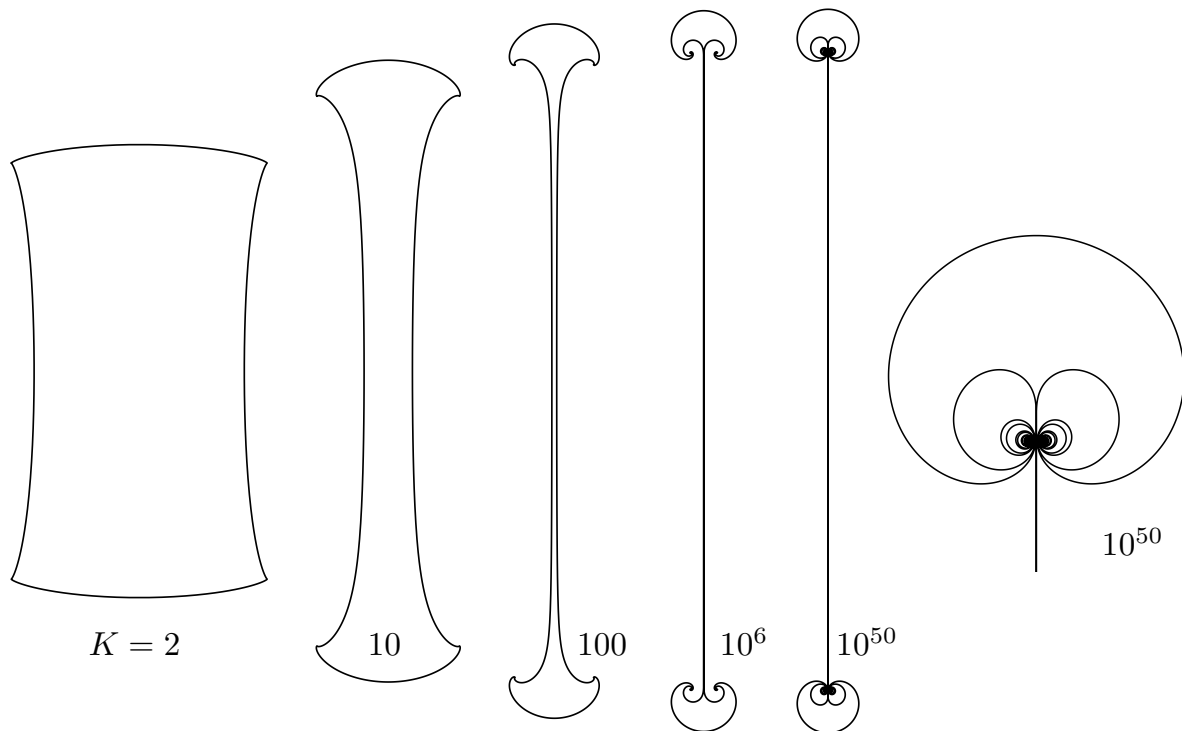
FIGURE 1. The image of the square by the straightening of the Beltrami form, for different values of K .
