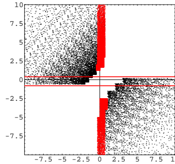
FIGURE 1. A typical attractor
