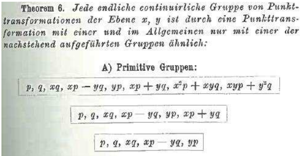
FIGURE 1. Fragment from [6, Page 71] (there the statement of the theorem continues).
