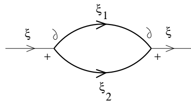
FIGURE 1. Bubble diagram. Boldface lines scale as 1/|\xi|^{1+2\alpha} .
