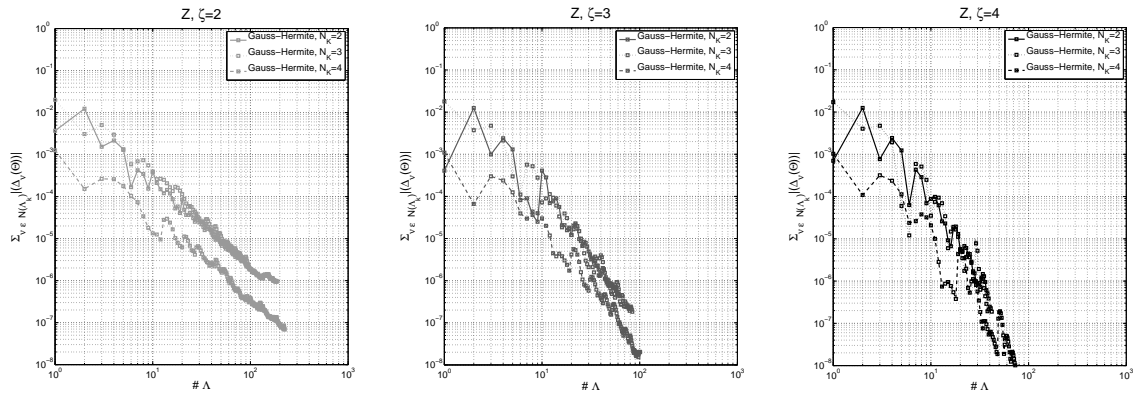
FIGURE 2. Comparison of the error curves of the normalization constant Z with respect to \#\Lambda_N based on the Gauss-Hermite quadrature with number of observations K = 2^{N_K} - 1 , N_K = 2, 3, 4 , \eta \sim \mathcal{N}(0, 1) and \zeta = 2 (l.), \zeta = 3 (m.) and \zeta = 4 (r.).
