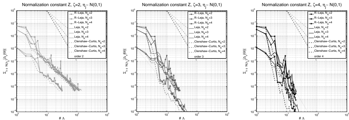
FIGURE 1. Comparison of the error curves of the normalization constant Z with respect to \#\Lambda_N based on the sequences with Clenshaw-Curtis, symmetrized Leja and R-Leja quadrature points with number of observations K = 2^{N_K} - 1 , N_K = 2, 3, 4 , \eta \sim \mathcal{N}(0, 1) and with \zeta = 2 (left), \zeta = 3 (middle) and \zeta = 4 (right).
