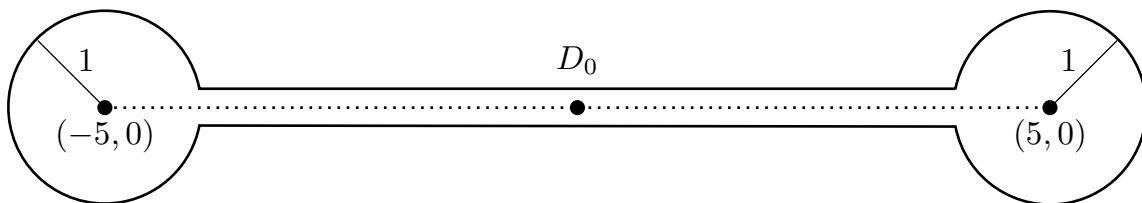
FIGURE 1. The dumbbell domain D_0 .
