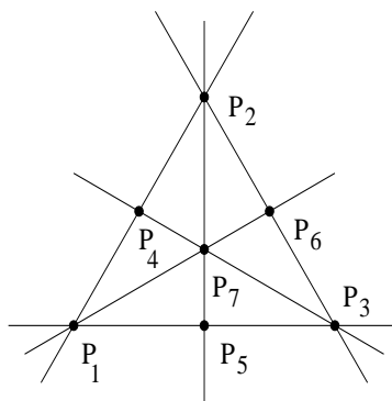
FIGURE 1. The A_3 -arrangement
