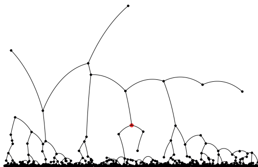
FIGURE 1. Simulation in the upper half-space model and added origin (red)
