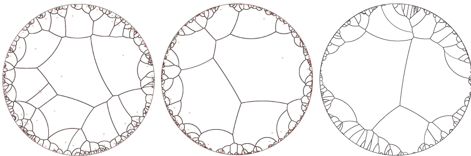
FIGURE 1. A simulation of three Poisson–Voronoi tessellations of \mathbb{H}^2 with intensity 1, 0.1 and 0.001. The limiting tessellation has no nuclei but still reveals an interesting geometry.
