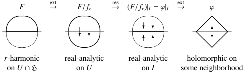
FIGURE 9. \rho_r^{\mathrm{pj}} as a sequence of extensions and restrictions.
