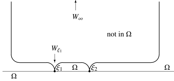
FIGURE 1. An \{\infty, \xi_1, \xi_2\} -excised neighborhood.
