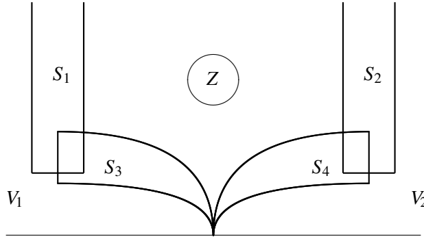
FIGURE 17. Illustration for the proof of Lemma 10.11. We take C = \sum_{j=1}^4 \varepsilon_j x_j . The singularities of \tilde{c}(x_j) are contained in S_j , and we can take U_j = \mathfrak{S} \setminus S_j . The union V_1 \cup V_2 is an excised neighborhood, on which \tilde{c}(C) represents c(C) .
