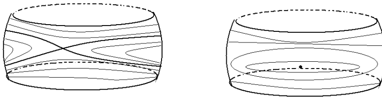
Figure 11: Hyperbolic singularity inside the cylinder. (Front and rear view)
