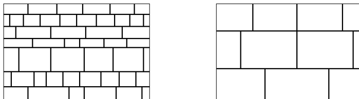
Figure 14: A brick wall cover, and one which is not
