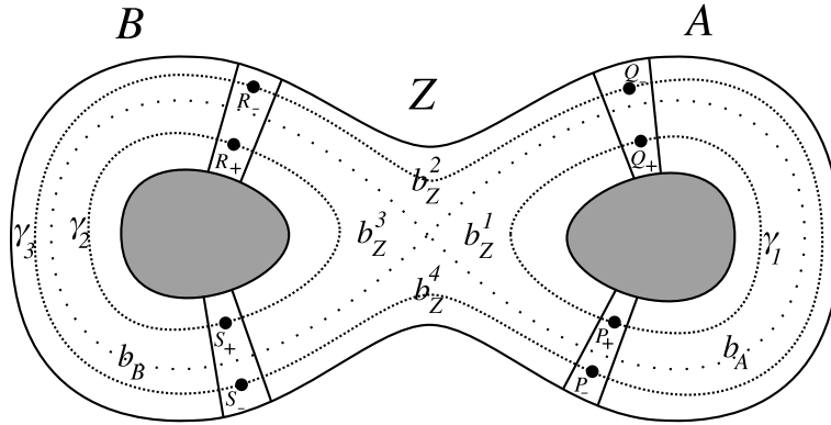
Figure 3: Diagram for the cohomology calculation
