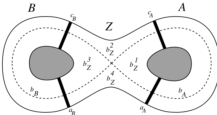
Figure 2: A simple cover of the figure-eight
