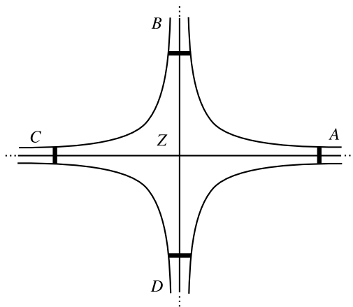
Figure 8: The covering near one hyperbolic singular point
