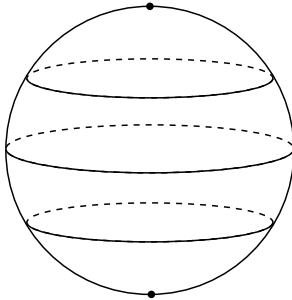
Figure 12: The height function on a sphere
