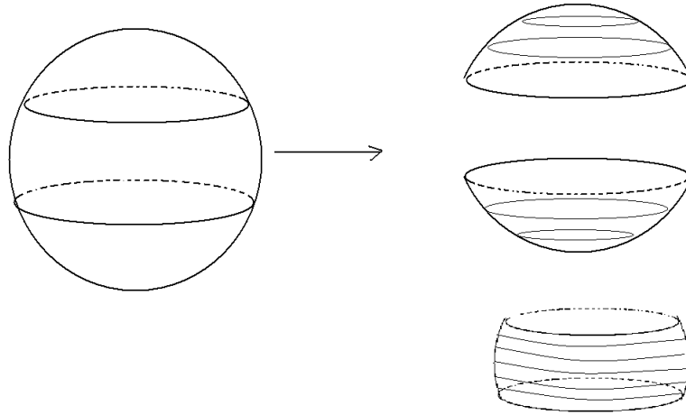
Figure 10: Cutting out a cylinder.
