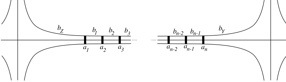
Figure 9: Leaf between two singular points
