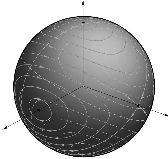
Figure 13: Reduced Hamiltonian flow of Euler's equations
