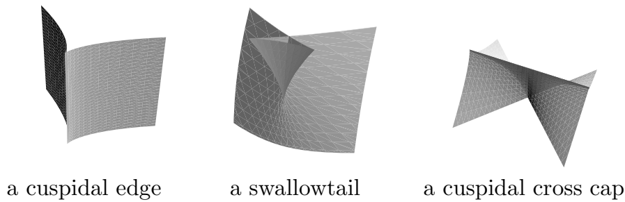
FIGURE 1. Generic singularities of CMC-1 faces
