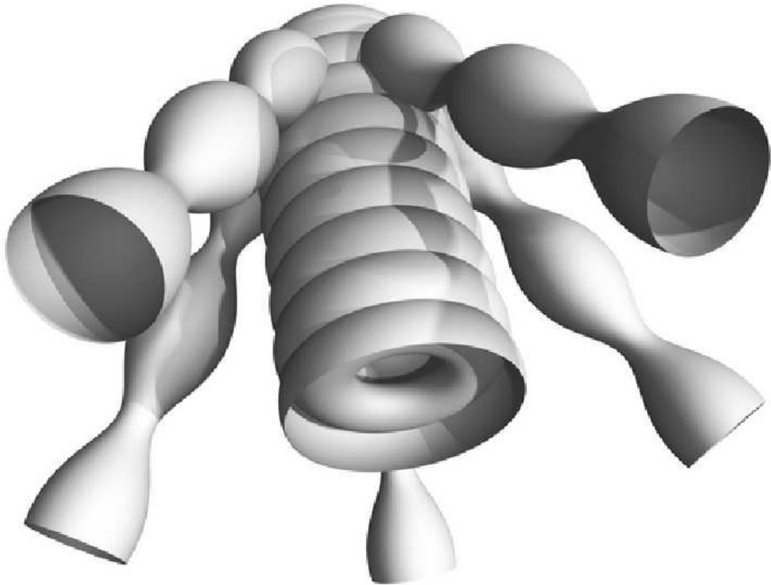
FIGURE 1. A CMC immersion of the six-punctured sphere with asymptotically Delaunay ends and pyramidal symmetry [15]. Five of the six ends are unduloidal; the sixth is nodoidal with large negative weight.
