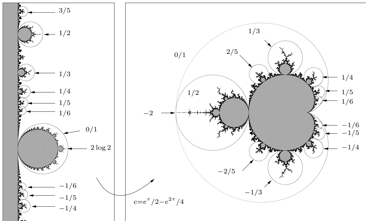
FIGURE 1. Geometric interpretation of the Pommerenke-Levin-Yoccoz inequality.
