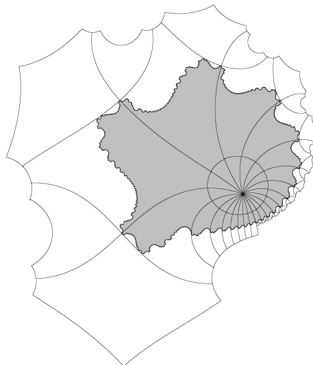
FIGURE 7. The open set U_1(\alpha) for \alpha = [10, 10, 10, \dots] .
