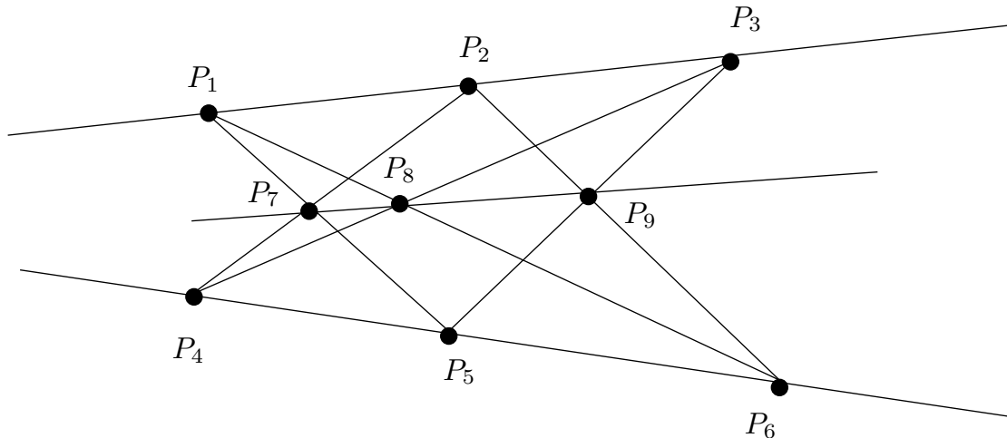
FIGURE 1. The Pappus configuration
