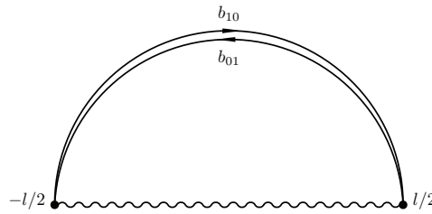
FIGURE 1. A Taub-NUT Bow Diagram.
