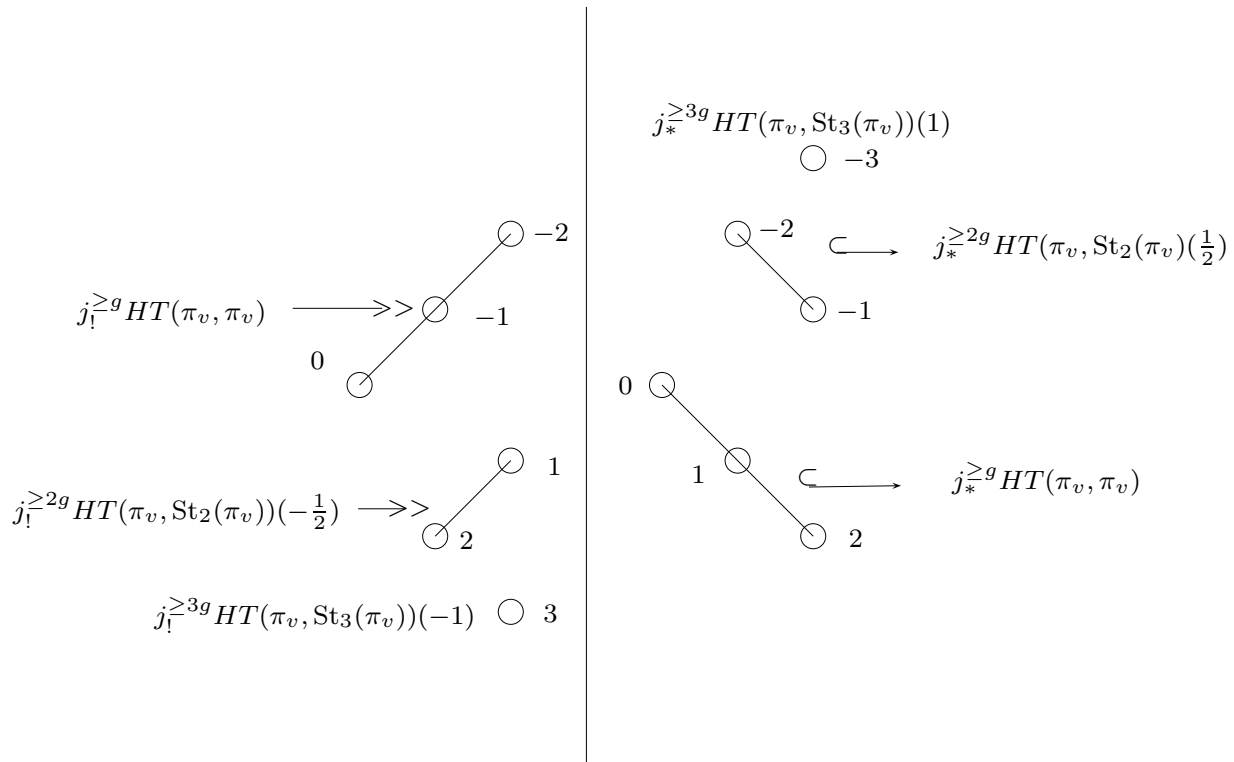
FIGURE 1. Filtration (fig. on the left) and cofiltration (fig. on the right) of stratification of \Psi_{\pi_v} with d = 3g .
