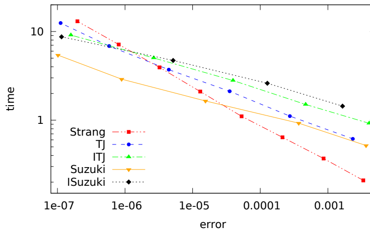
FIGURE 3. Work-precision plot (using the discrete infinity norm) for the KdV equation with the sech soliton initial value integrated up to T = 0.05 with 2^{10} grid points.
