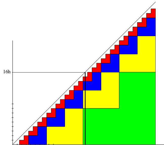
FIGURE 2. Splitting of the t - \tau plane.
