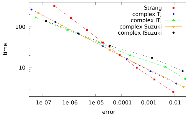
FIGURE 2. Work-precision plot (using the discrete infinity norm) for the Brusselator integrated up to T = 0.25 with 2^{10} grid points per dimension (in total we have 2^{21} grid points).
