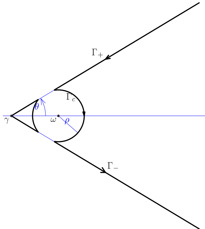
FIGURE 1. The K -spectral set X .
