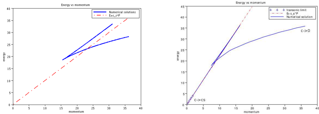
FIGURE 2. E-P diagram for : Left, a cubic-quintic-septic nonlinearity; Right: a saturated exponential nonlinearity.
