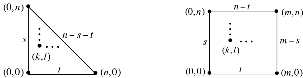
FIGURE 2. Polygons with three and four sides.
