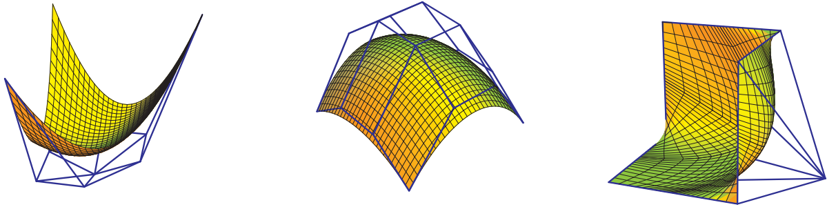
FIGURE 1. Toric Bézier patches
