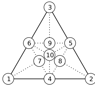
The 12-split with numbering of vertices.
