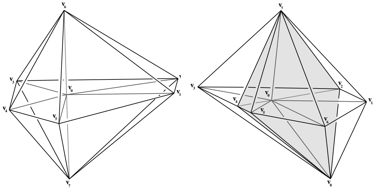
FIGURE 1. Collinear (left) and coplanar II (right) cases
