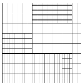
FIGURE 1. A mesh obtained by partially nested hierarchical spline refinement.
