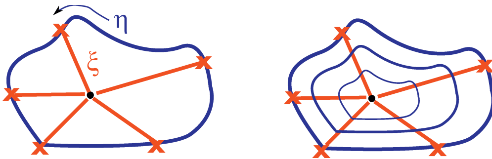
FIGURE 1. Sketch of polar coordinate system and isogeometric mesh
