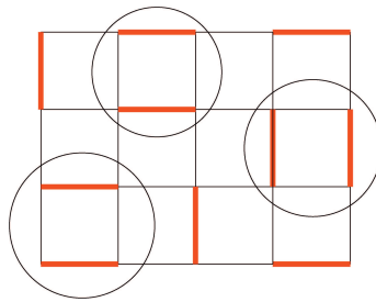
FIGURE 2. A dimer configuration D covering a finite portion of the square lattice, and the plaquettes such that N_P(D) = 1 .
