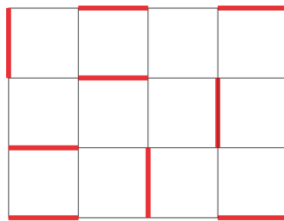
FIGURE 1. An example of an admissible dimer configuration on a finite portion of the 2D square lattice.
