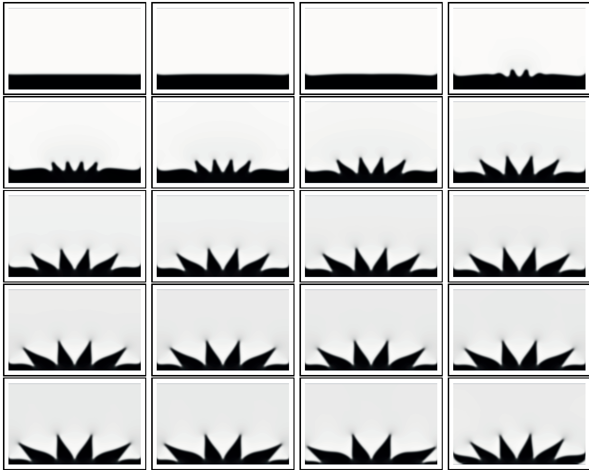
FIGURE 1. The Rosensweig instability
