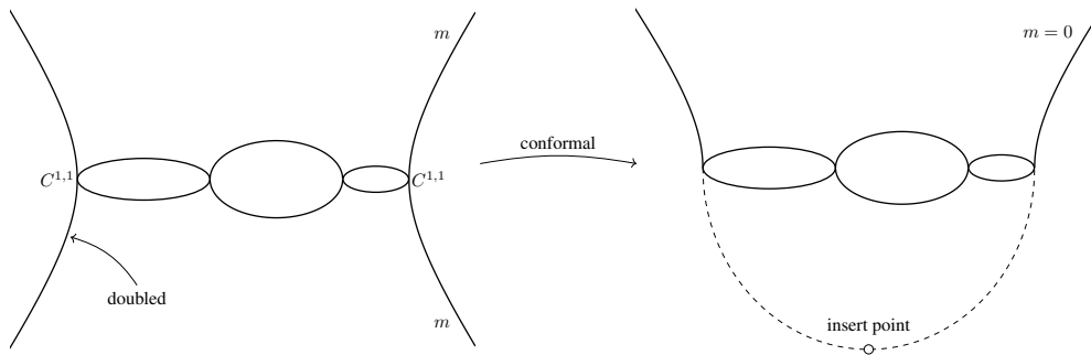
FIGURE 3. Conformal transformation and one-point insertion to a geodesically complete Riemannian manifold with vanishing ADM-mass and non-negative scalar curvature.
