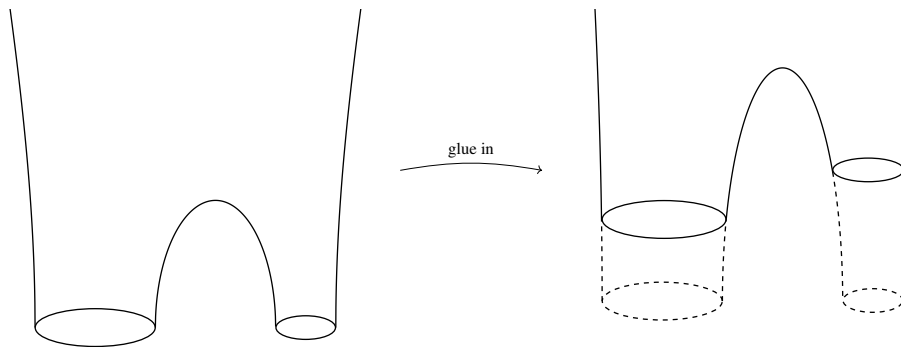
FIGURE 1. Gluing in a suitable, explicitly constructed Riemannian manifold (M_i^n, g_i) into each inner boundary component \Sigma_i^{n-1} . The new boundary components are totally geodesic semi-static horizons.
