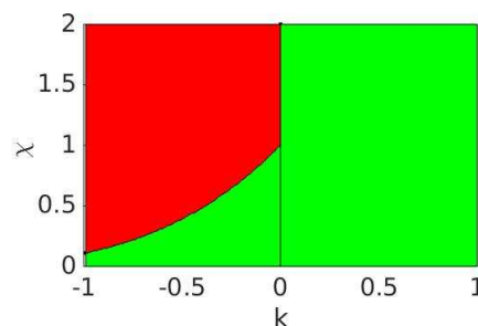
FIGURE 1. Regions of blow up (red) and convergence to self-similarity (green) in 1D.
