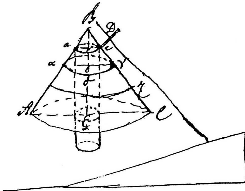
FIGURE 1. Hermann's planimeter: sketch from a manuscript, c1814/1815
