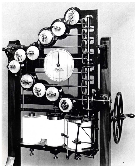
FIGURE 2. Tide Predictor (1876), Science Museum London SSPL. Inv. 1896-60
