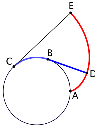
FIGURE 1. Involute of a circle. A string wrapped around ABC , unwrapped from D
