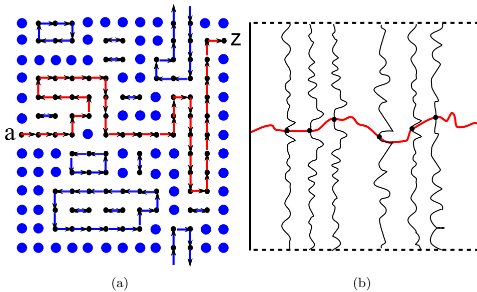
FIGURE 1. (a) : Representation of a bijection with a forced open cycle between a and z , when \Lambda \subset \mathbb{Z}^2 is a box with cylinder boundary conditions. If \pi(x) = x , then a circle is drawn at x , while if \pi(x) is a neighbour of x , then an arrow is directed from x to \pi(x) . (b) : Regeneration interfaces intersect the forced open cycle at regeneration points, which are represented by small black circles.
