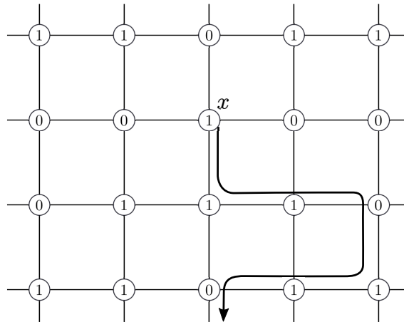
FIGURE 1. The word 1110110... is read from x .
