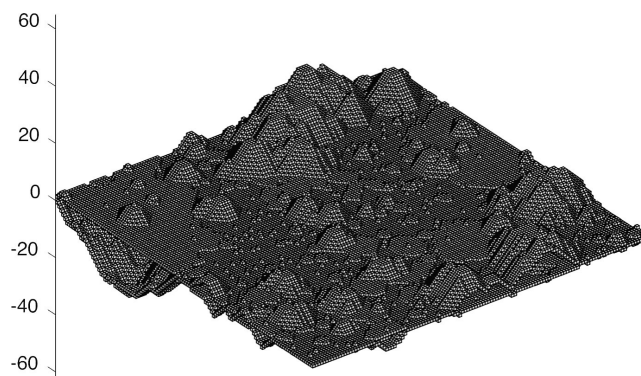
FIGURE 1. Two-sided Lipschitz surface on \mathbb{Z}^3
