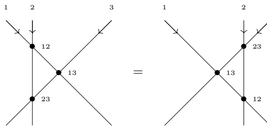
FIGURE 1. Graphical representation of the Yang-Baxter equation.
