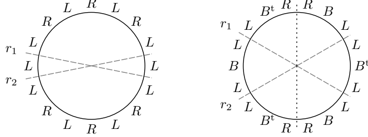
FIGURE 7. Diagrams with two para-symmetries
