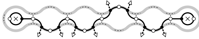
FIGURE 12. A junction of six M -cubics (*\uparrow\uparrow\downarrow\uparrow*)
