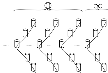
FIGURE 2. Auslander-Reiten quiver of \text{coh } X
