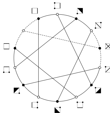
FIGURE 1. The diagonal link of NCP_4 inside the incidence graph of the Fano plane.
