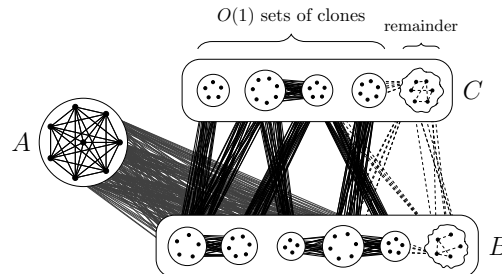
FIGURE 2. Structure of G
