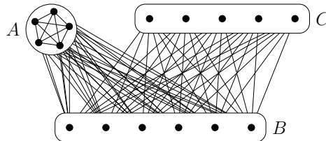
FIGURE 1. The graph G(a, b, c)
