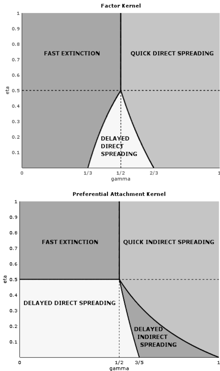
FIGURE 1. The figures summarise the theorem in the form of phase diagrams for the factor kernel (top) and the preferential attachment kernel (bottom).
