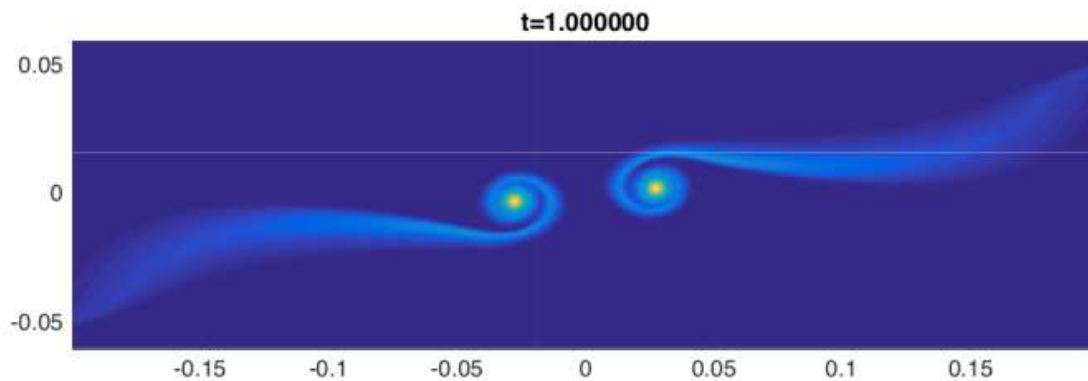
FIGURE 3. A symmetric solution containing two spirals. This depicts the solution to (1) at time t = 1 , with initial data (9) with \varepsilon > 0 small. Here \mu = 5/7 .
