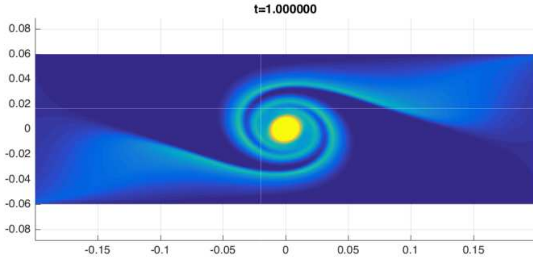
FIGURE 2. A single symmetric spiral. This depicts the solution to (1) at time t = 1 , with initial data (8) with \varepsilon > 0 small. Here \mu = 5/7 .
