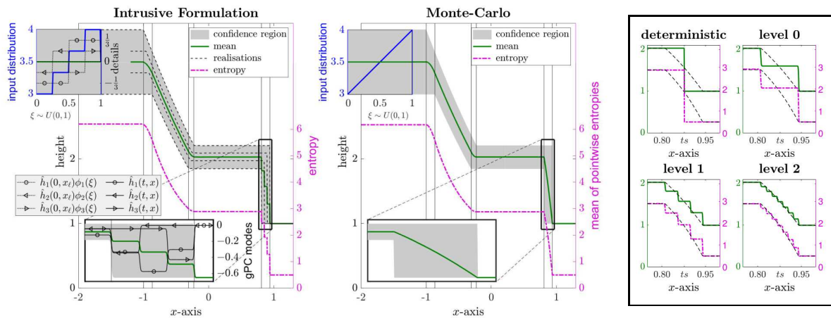
FIGURE 1. Dam break problem in t = 0.5 with uniformly distributed left initial value
