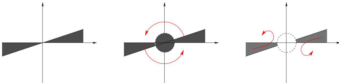
FIGURE 1. The supports of the initial vorticity. Left: the original datum (6). Center: the approximation (8). Right: the approximation (9).
