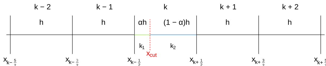
FIGURE 1. Model problem: Equidistant mesh with one cell, cell k , split into two cells of lengths \alpha h and (1 - \alpha)h with \alpha \in (0, \frac{1}{2}] .
