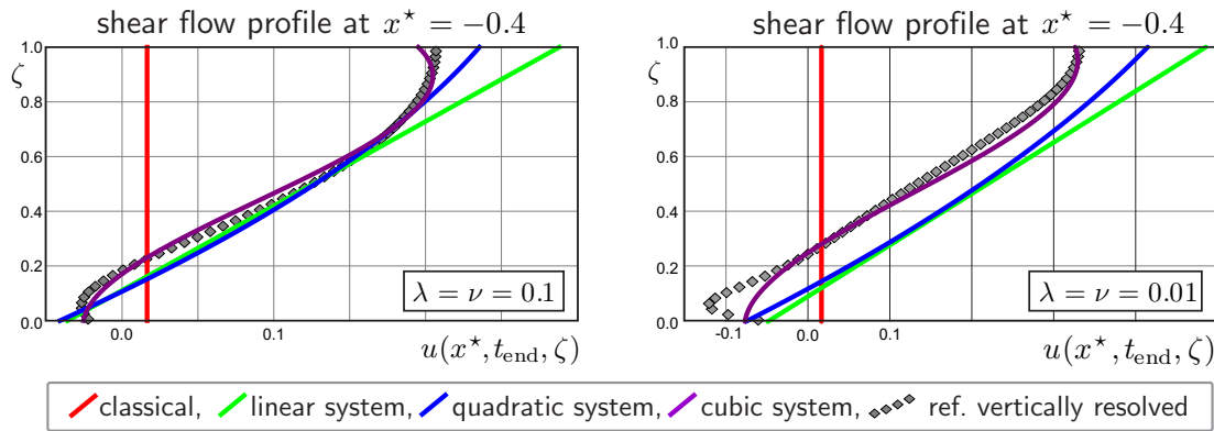
FIGURE 1. Approximation of a vertical velocity profile with successive moment models of shallow flow. Symbols are obtained from a vertically resolved reference solution. The linear model corresponds to N = 1 , the quadratic model to N = 2 , etc.
