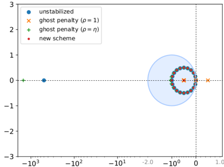
FIGURE 2. Distribution of eigenvalues for the three spatial discretizations described in (2), (3), and (4).
