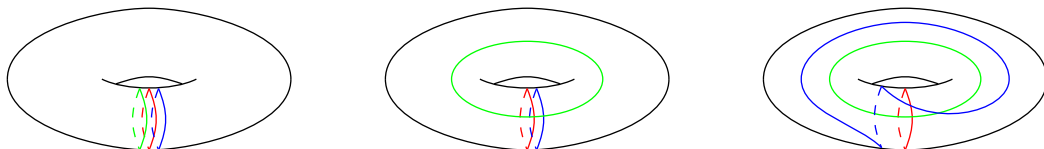
FIGURE 3. Genus one trisection diagrams
