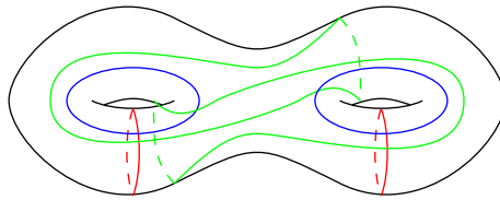
FIGURE 1. A trisection diagram
