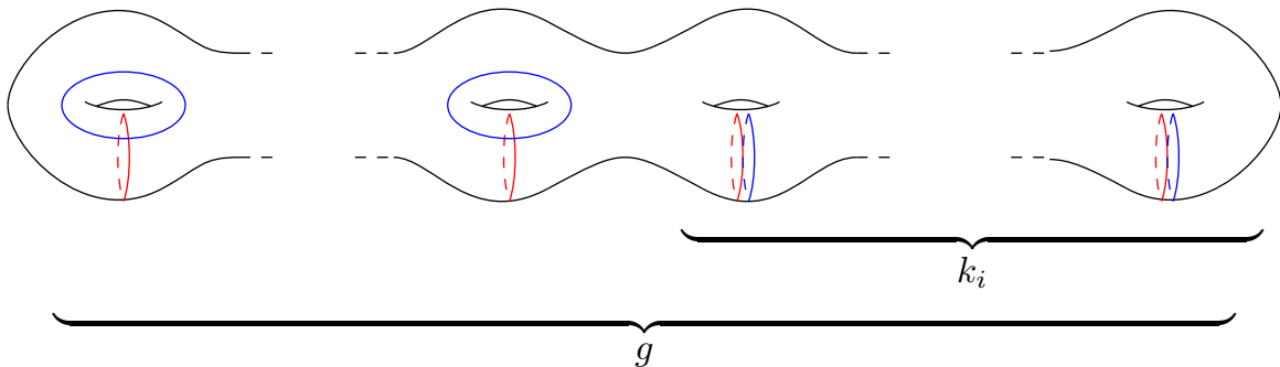
FIGURE 2. Genus- g Heegaard diagram for \sharp^{k_i} S^1 \times S^2
