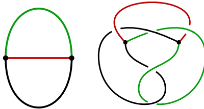
FIGURE 1. The trivial and Kinoshita \theta -curves with edges coloured.
