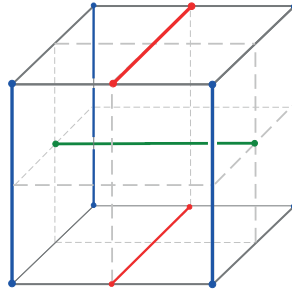
FIGURE 2. The candidate for the link L realising \text{volt}(\mathbb{T}^3) (from [9])
